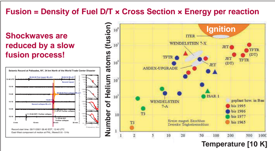
Source: https://en.wikipedia.org/wiki/Lawson_criterion
